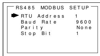
Figure 8-5: RS-485 MODBUS Setup Menu
