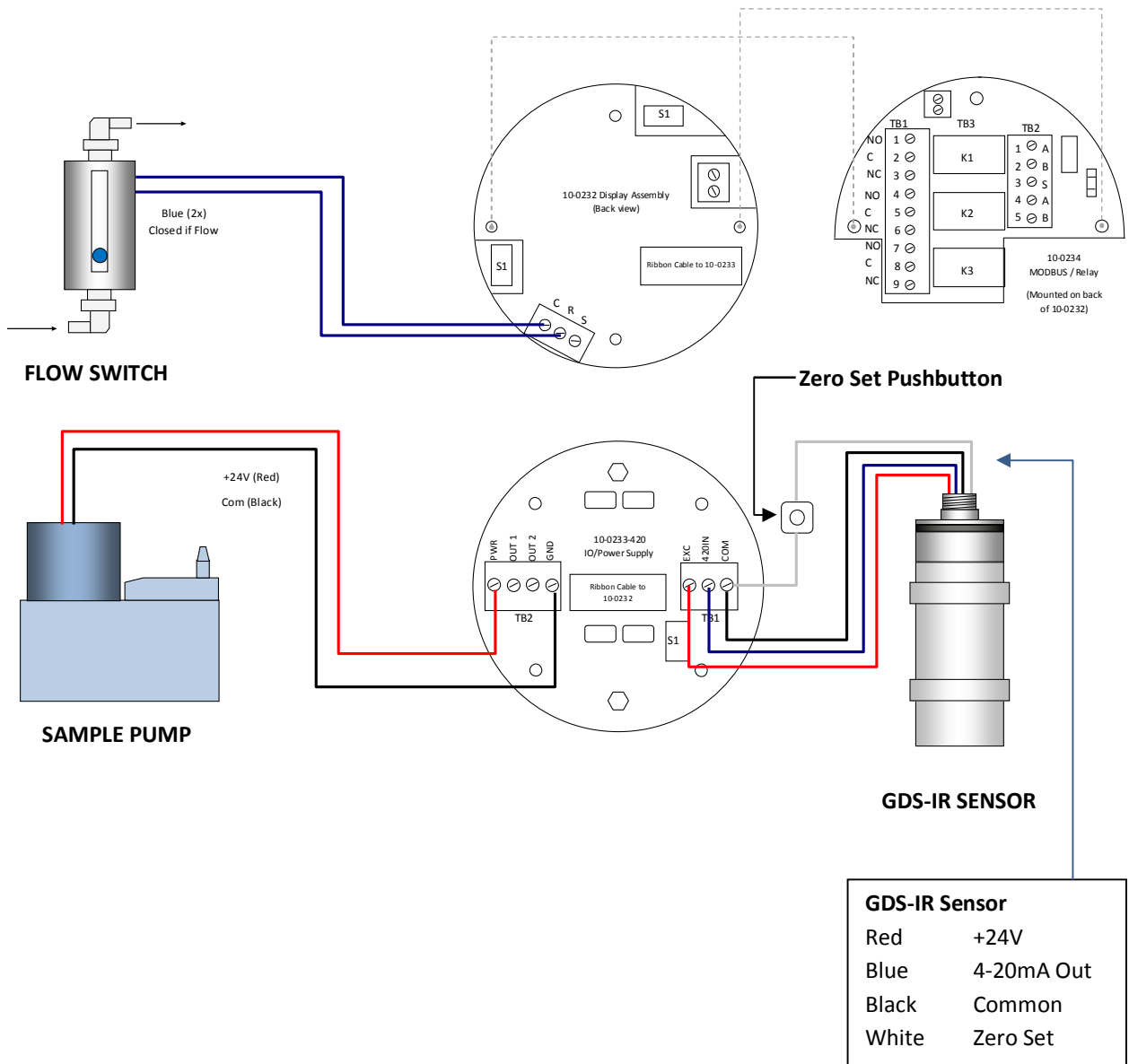
Figure 14-3: GDS-58XP Wiring Diagram (GDS-IR Sensor)
