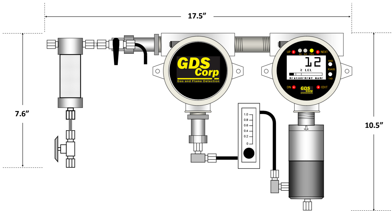
Figure 13-7: GDS-58XP with Optional Clear Coalescing Filter
