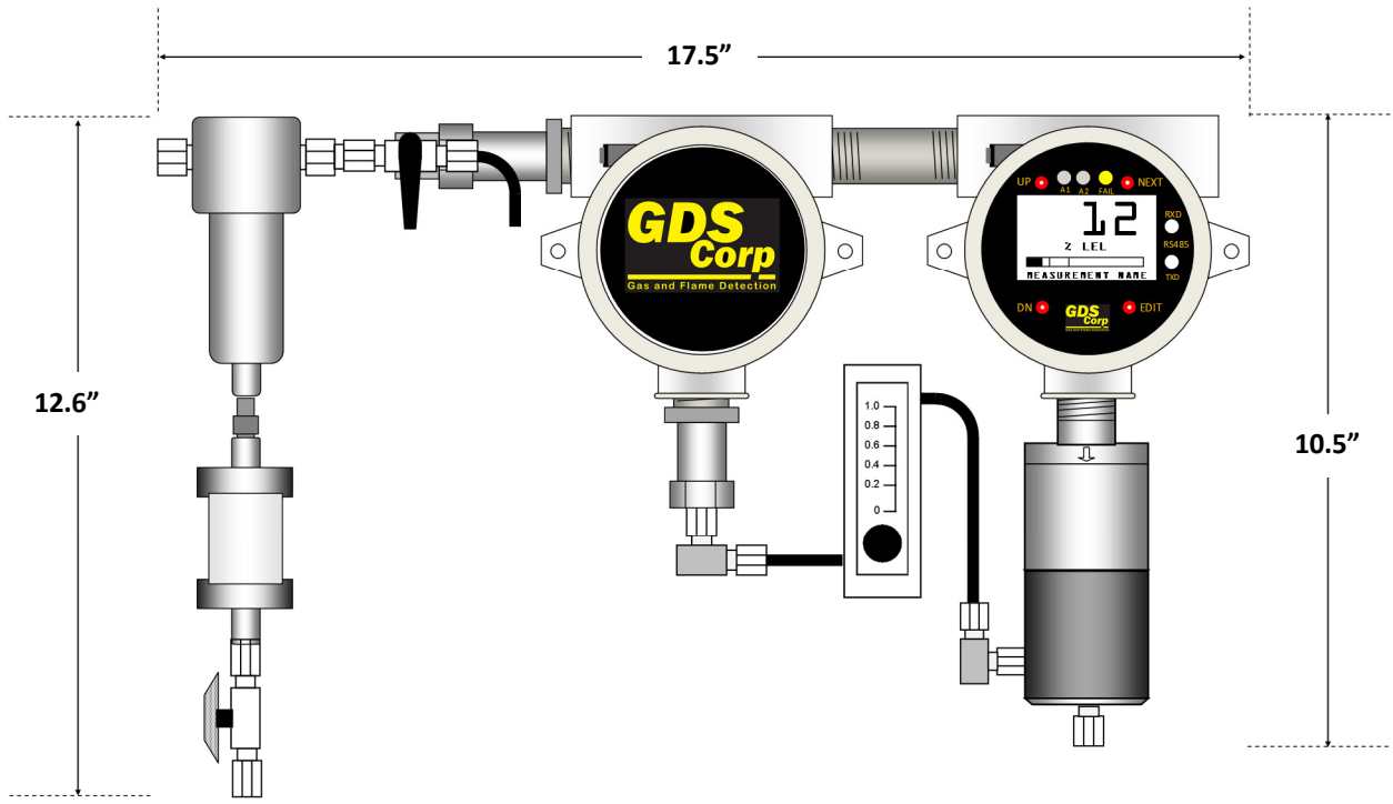
Figure 13-6: GDS-58XP with Optional Stainless Steel Coalescing Filter
