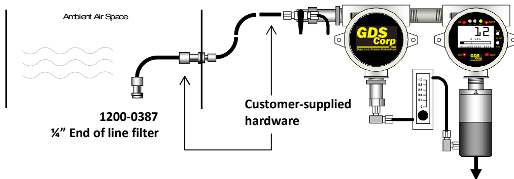
Figure 5-1: GDS-58XP Ambient Air Sampling
