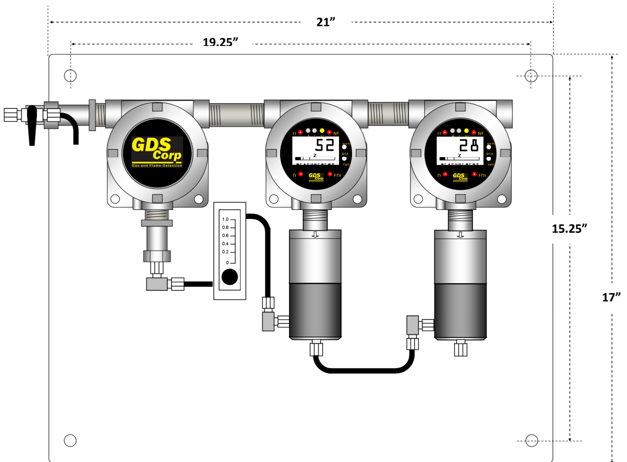
Figure 13-5: GDS-58XP 21" x 17" Mounting Plate Dimensions (SS Enclosures)
