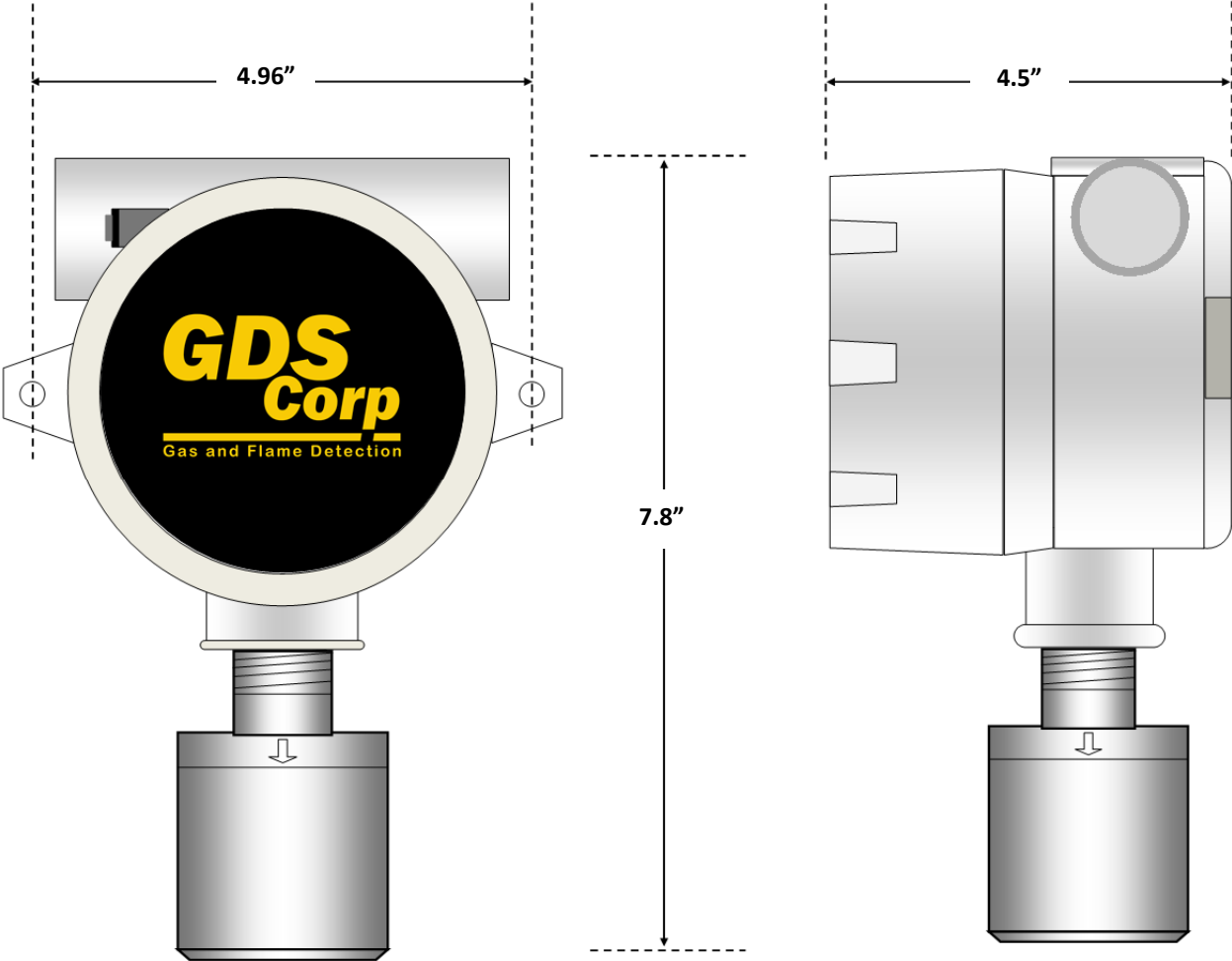
Figure 8-1: GDS-50 Dimensions
